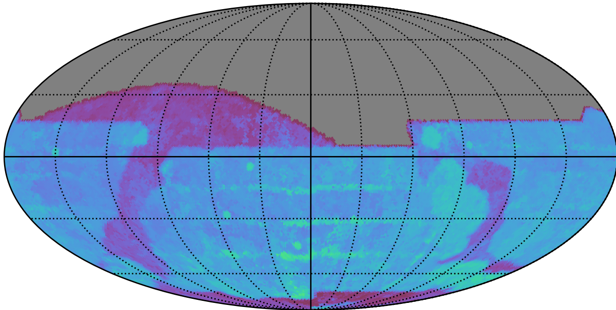
baseline_v3.0_10yrs All sky i band: 80thPercentile Season Length
