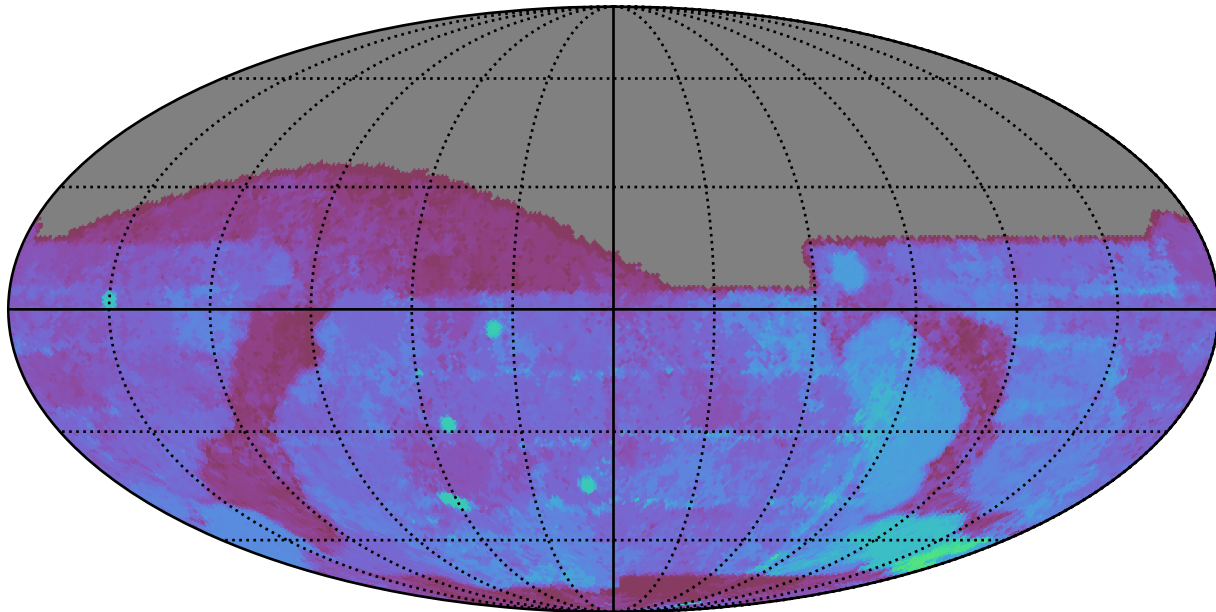
baseline_v3.0_10yrs All sky g band: 80thPercentile Season Length
