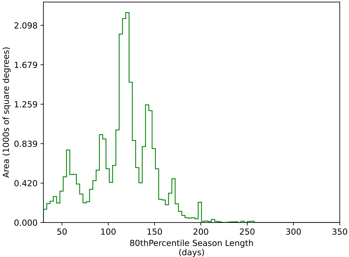
baseline_v3.0_10yrs All sky g band: 80thPercentile Season Length
