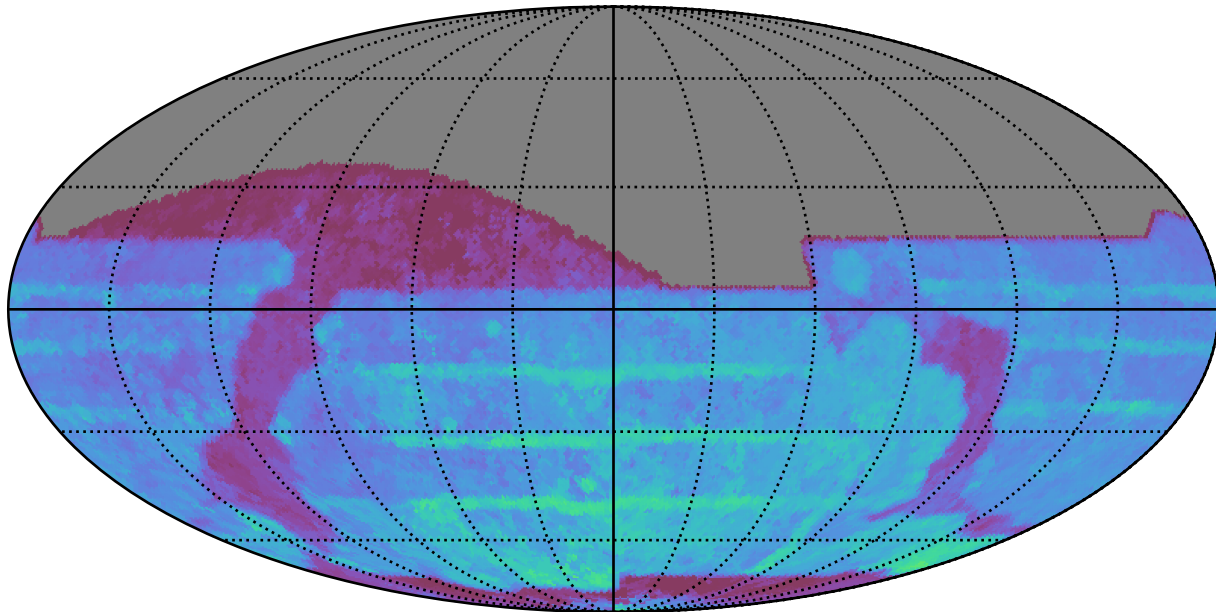
baseline_v3.0_10yrs All sky all bands: 80thPercentile Season Length
