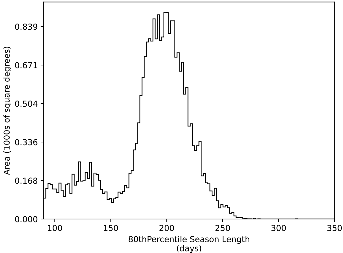
baseline_v3.0_10yrs All sky all bands: 80thPercentile Season Length
