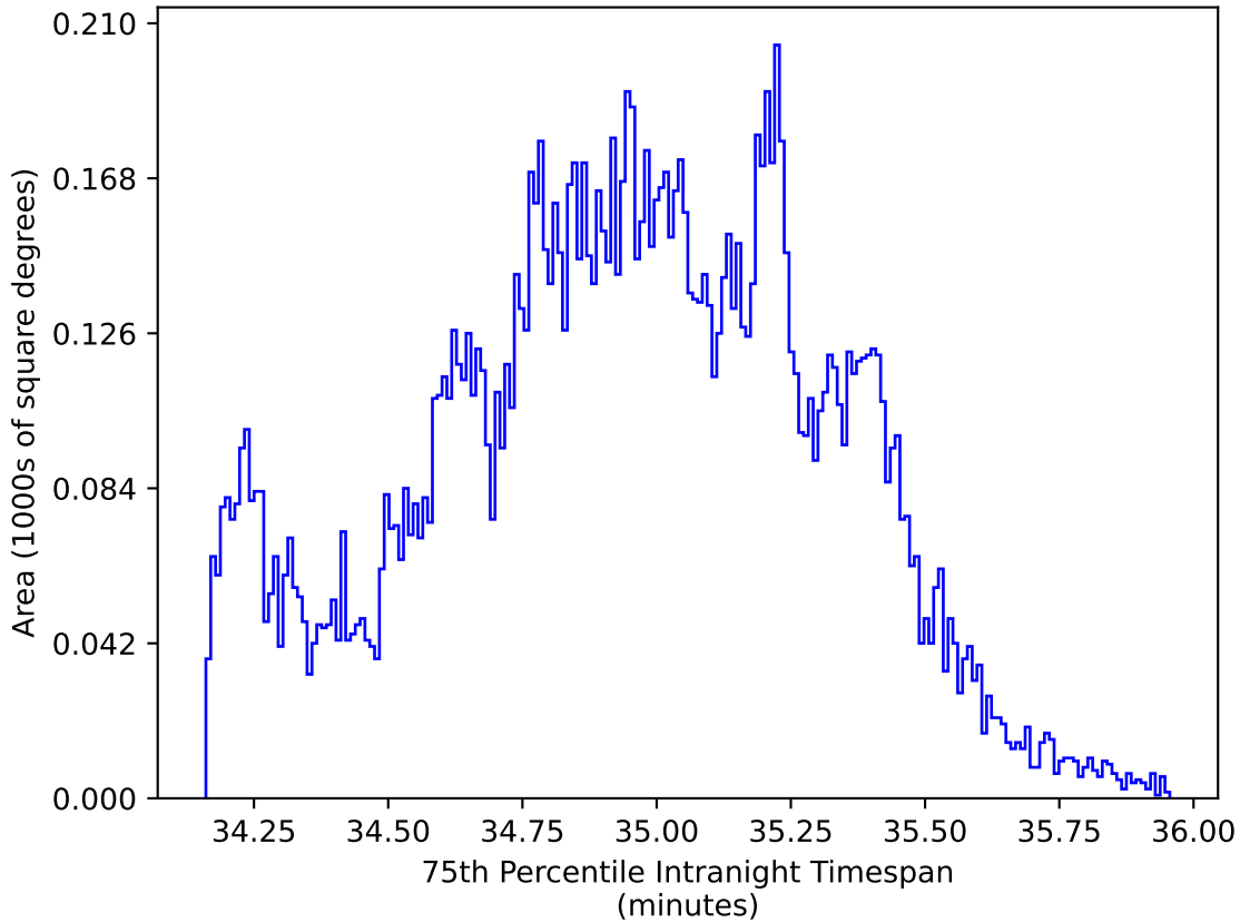
baseline_v3.0_10yrs WFD zy bands: 75th Percentile Intranight Timespan
