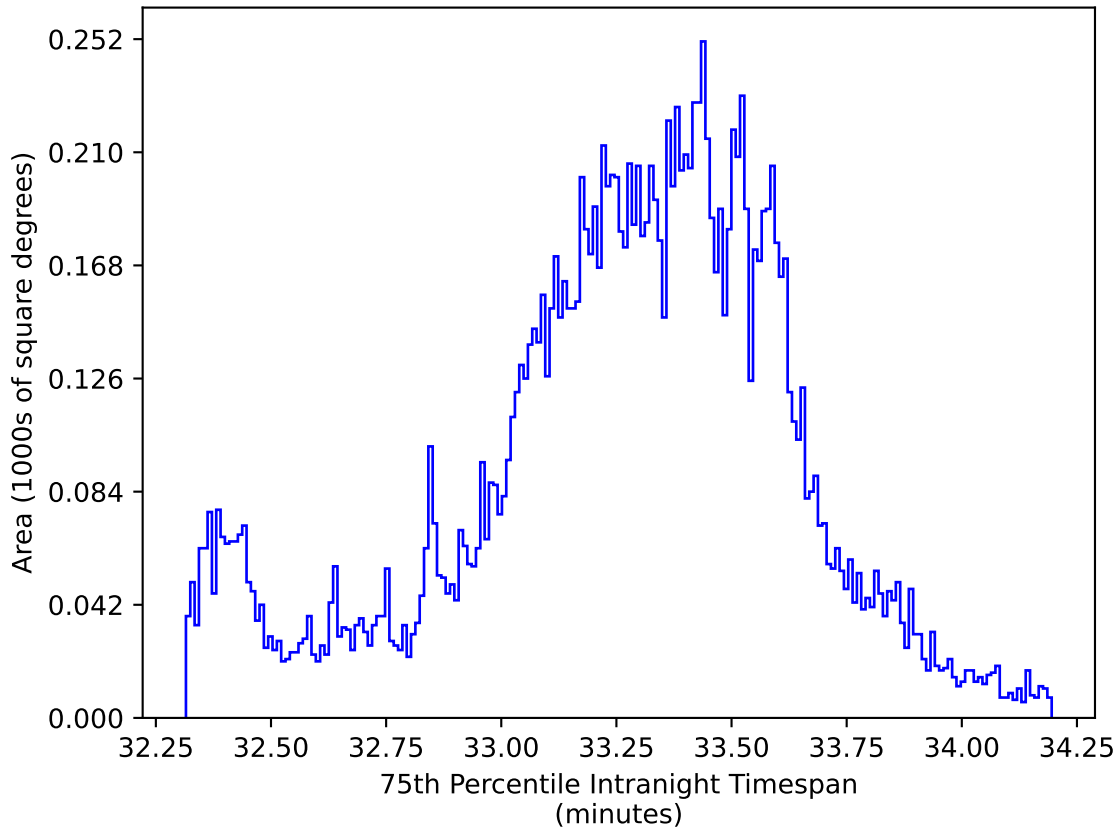
baseline_v3.0_10yrs WFD y band: 75th Percentile Intranight Timespan
