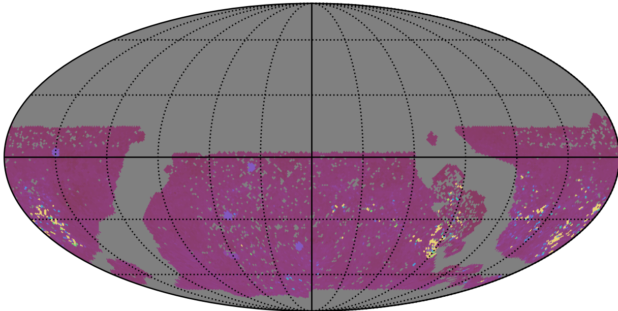
baseline_v3.0_10yrs WFD ug bands: 75th Percentile Intranight Timespan
