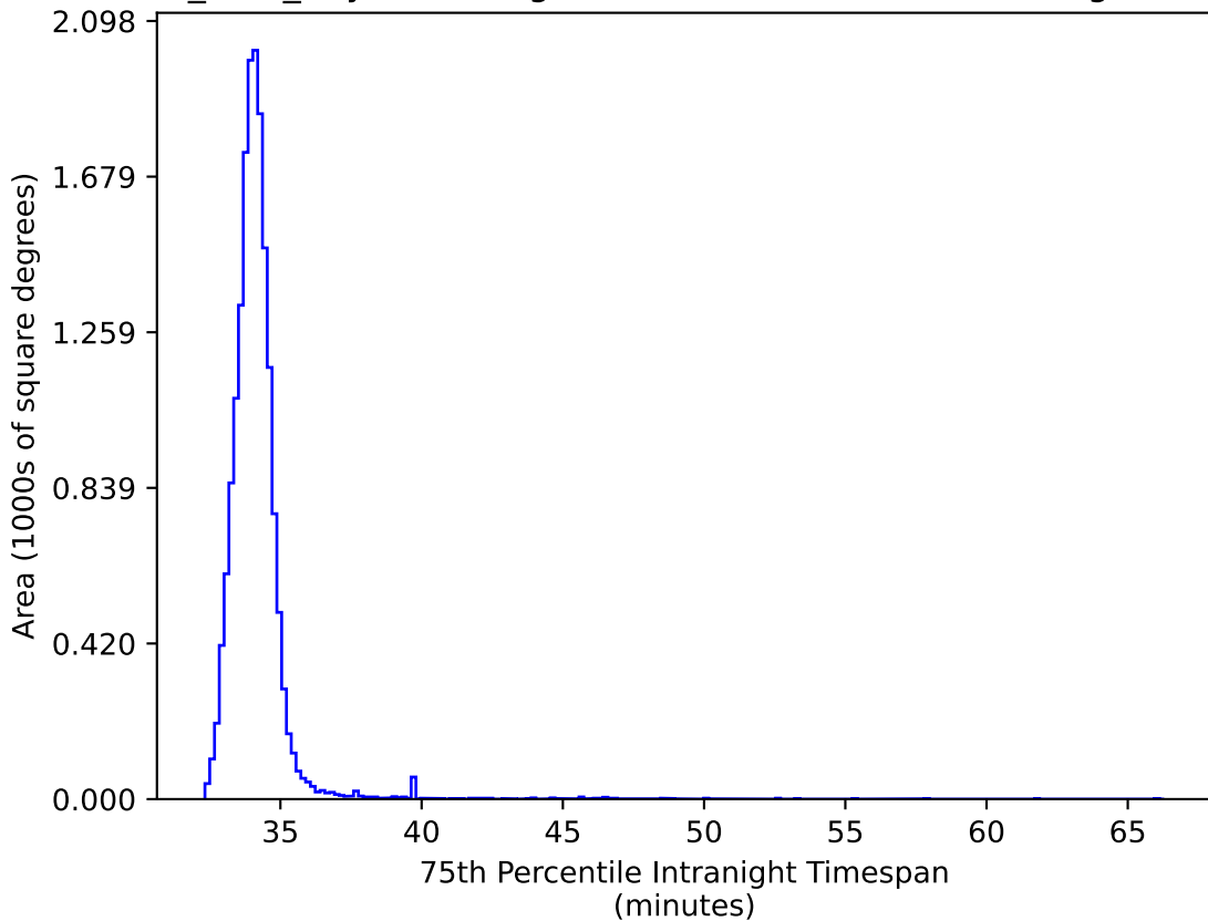
baseline_v3.0_10yrs WFD ug bands: 75th Percentile Intranight Timespan
