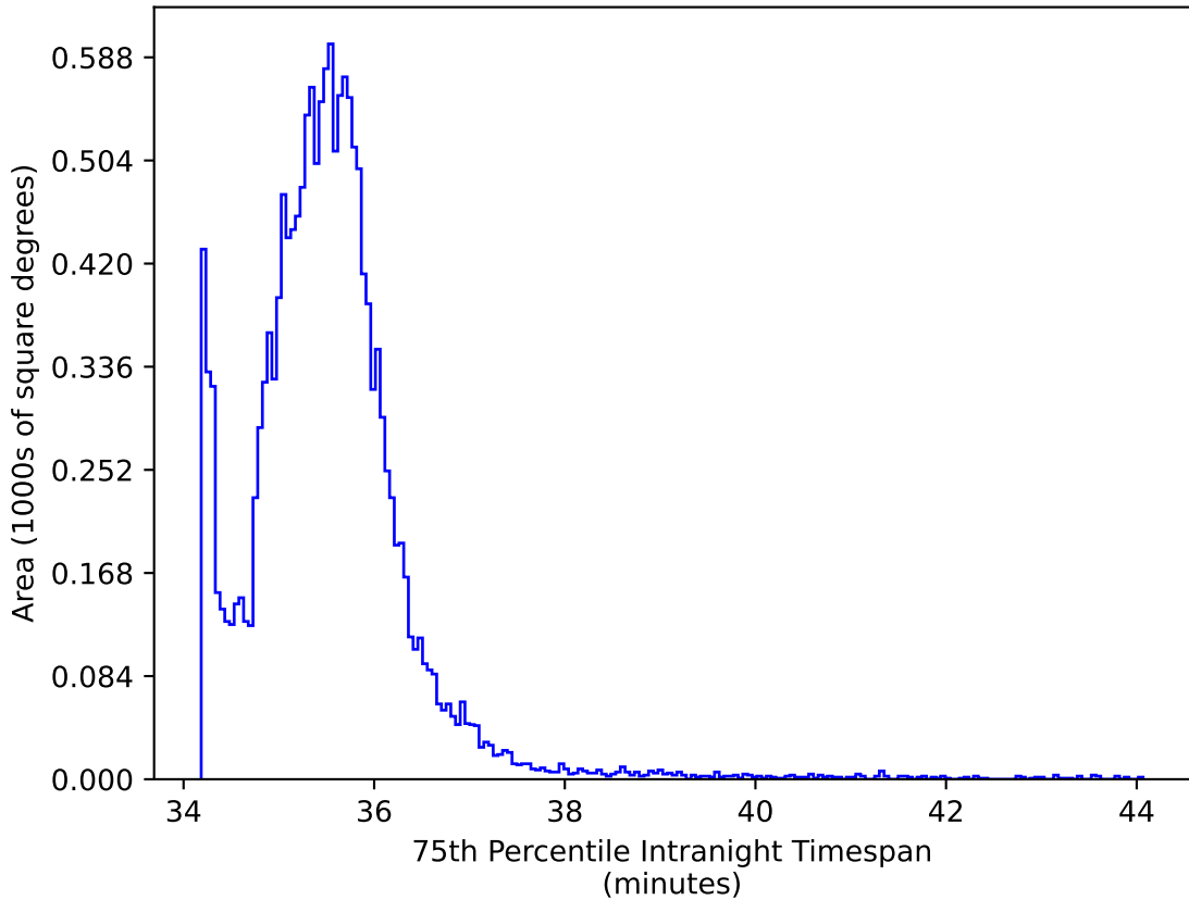
baseline_v3.0_10yrs WFD ri bands: 75th Percentile Intranight Timespan
