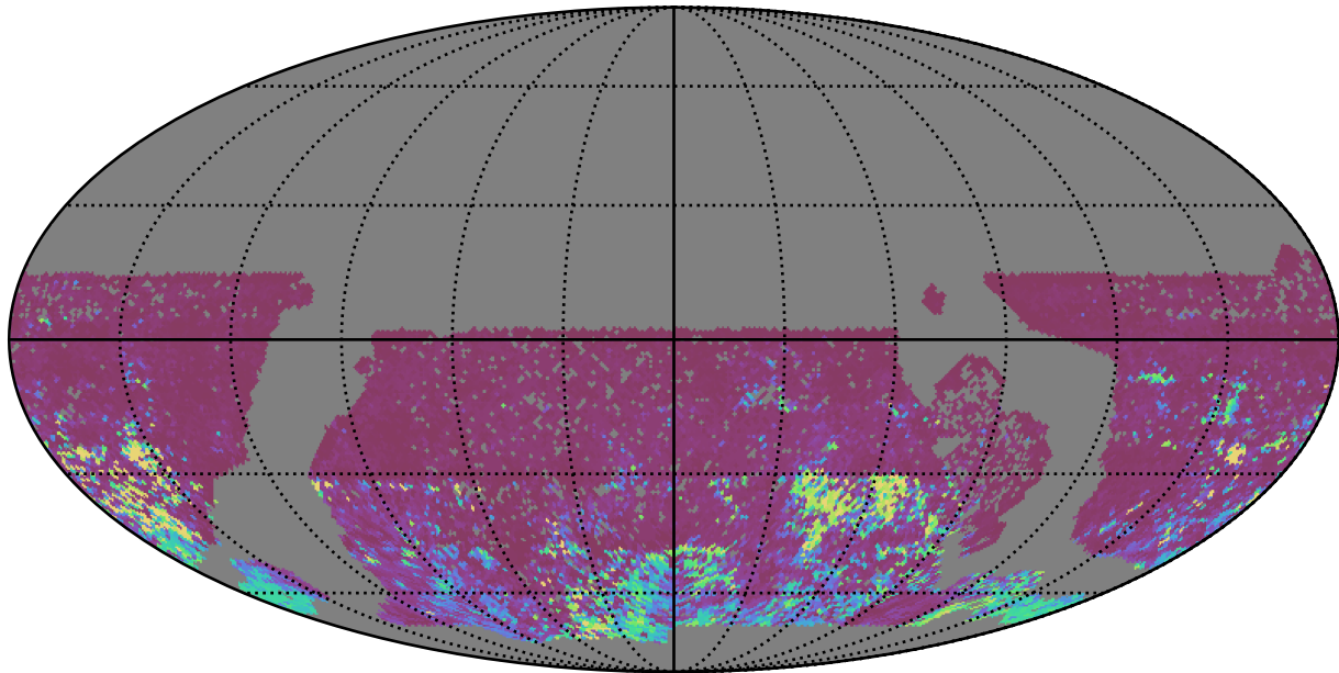
baseline_v3.0_10yrs WFD i band: 75th Percentile Intranight Timespan
