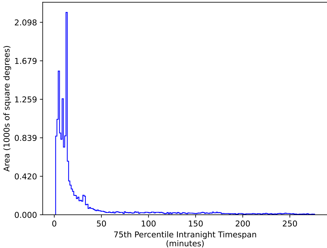
baseline_v3.0_10yrs WFD i band: 75th Percentile Intranight Timespan
