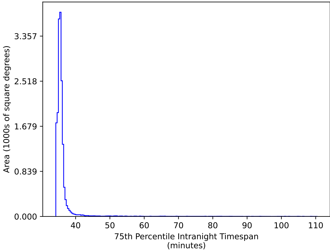
baseline_v3.0_10yrs WFD gr bands: 75th Percentile Intranight Timespan
