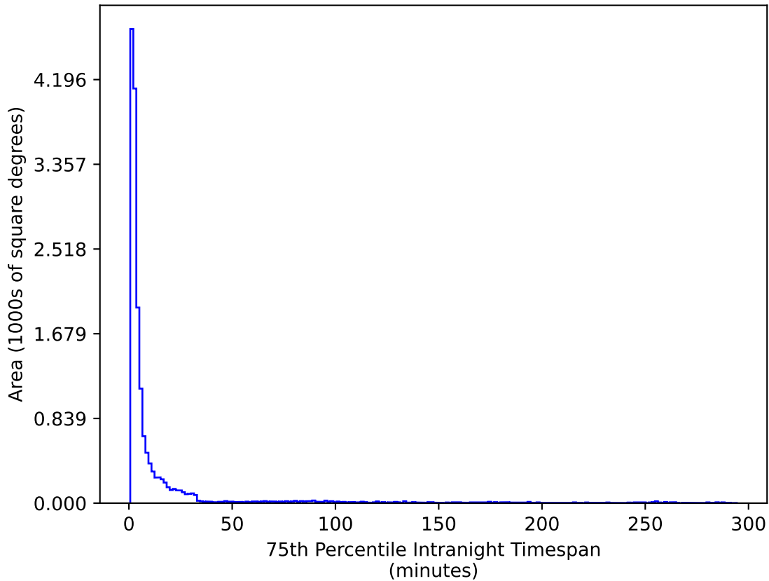
baseline_v3.0_10yrs WFD g band: 75th Percentile Intranight Timespan
