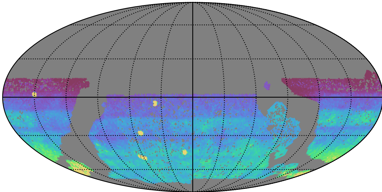
baseline_v3.0_10yrs WFD all bands: 75th Percentile Intranight Timespan
