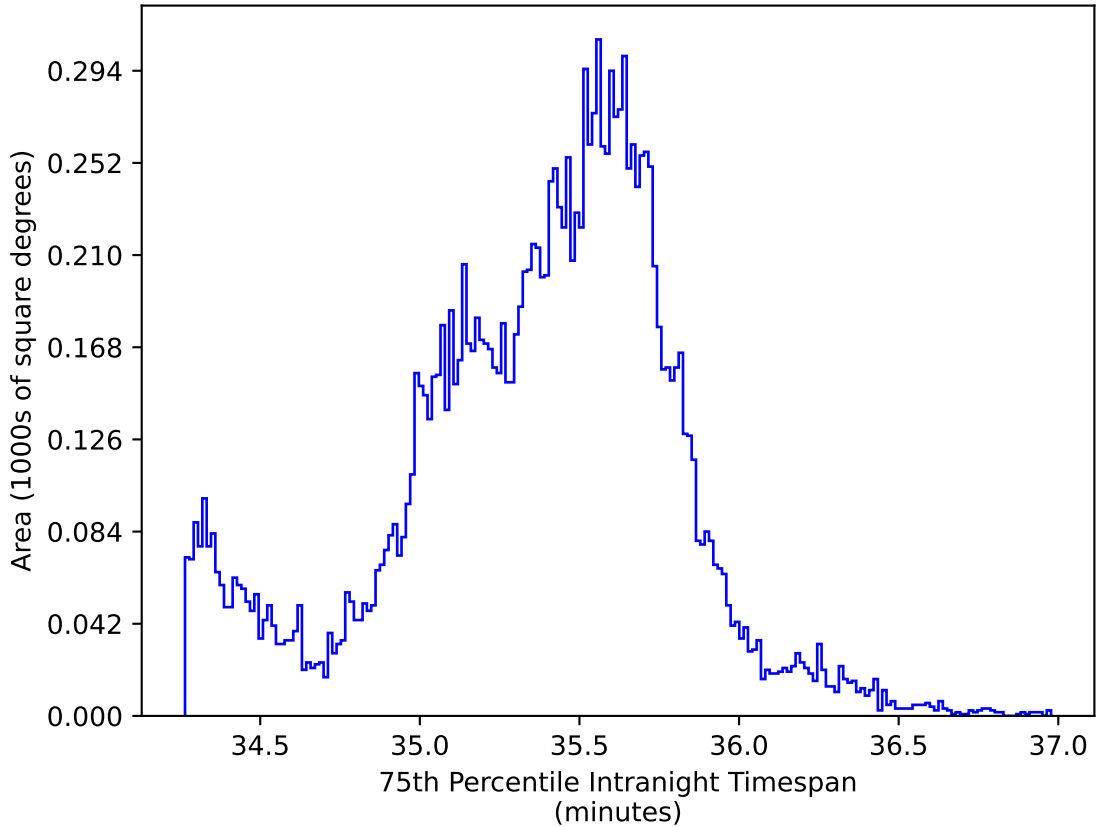
baseline_v3.0_10yrs WFD all bands: 75th Percentile Intranight Timespan
