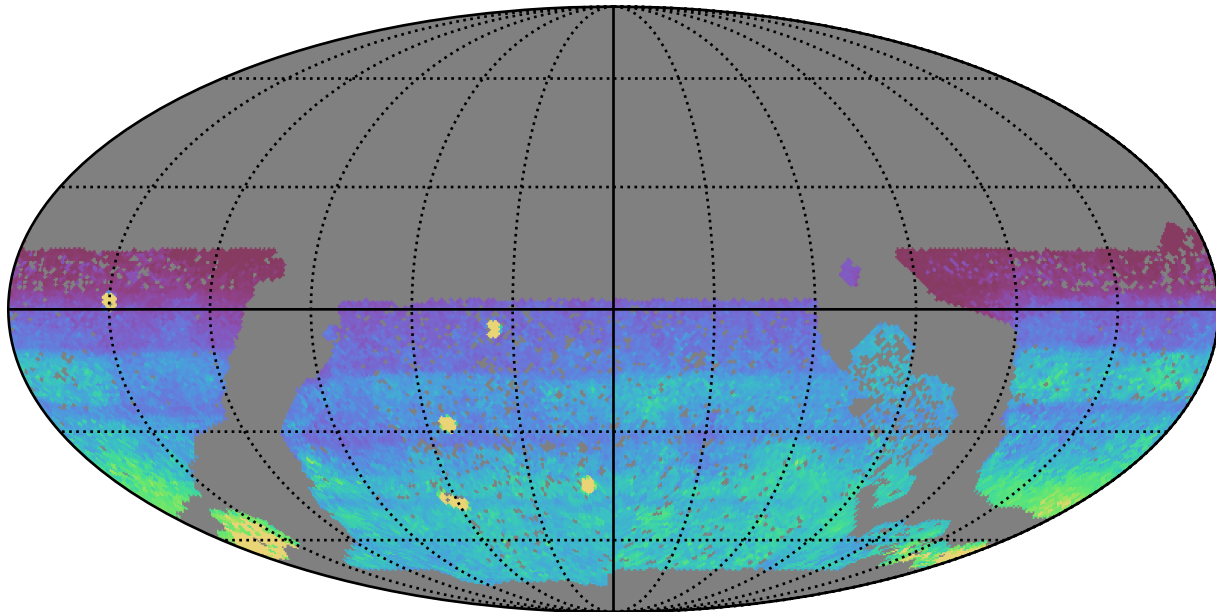
baseline_v3.0_10yrs WFD: 75th Percentile Intranight Timespan
