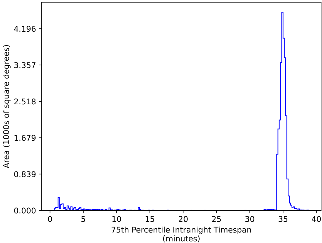
baseline_v3.0_10yrs All sky zy bands: 75th Percentile Intranight Timespan
