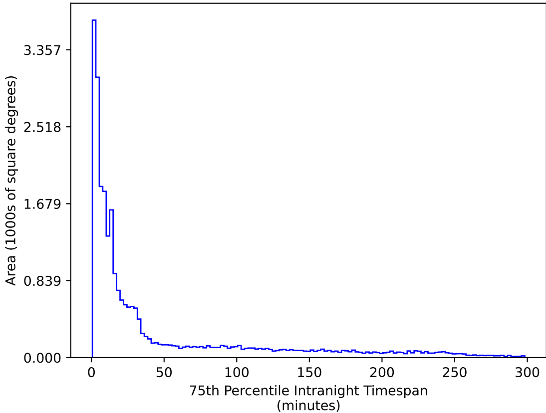
baseline_v3.0_10yrs All sky z band: 75th Percentile Intranight Timespan
