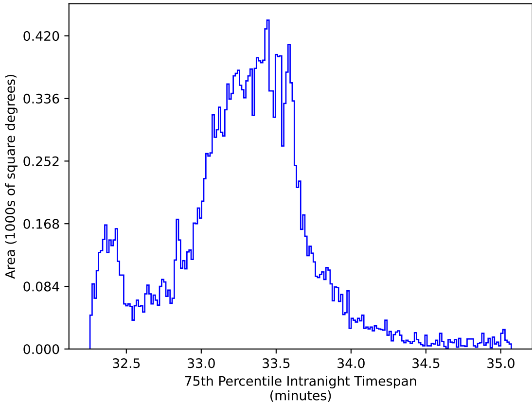
baseline_v3.0_10yrs All sky y band: 75th Percentile Intranight Timespan
