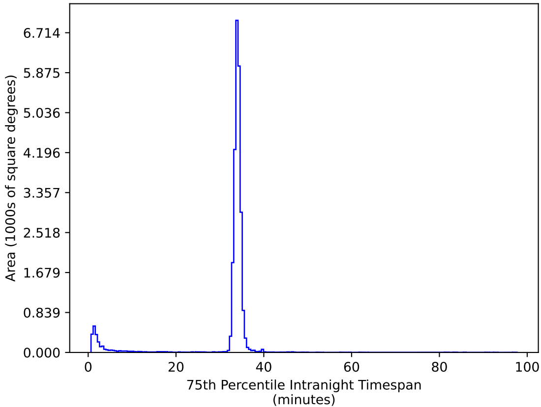
baseline_v3.0_10yrs All sky ug bands: 75th Percentile Intranight Timespan
