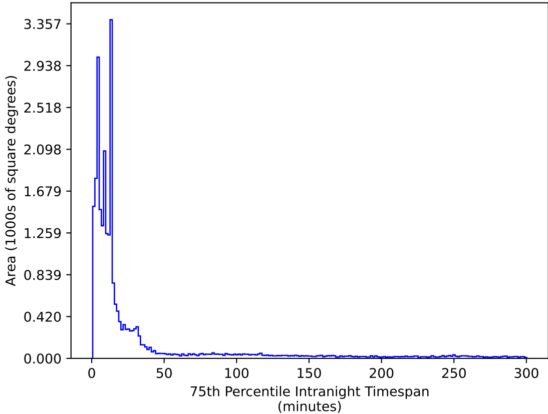
baseline_v3.0_10yrs All sky r band: 75th Percentile Intranight Timespan
