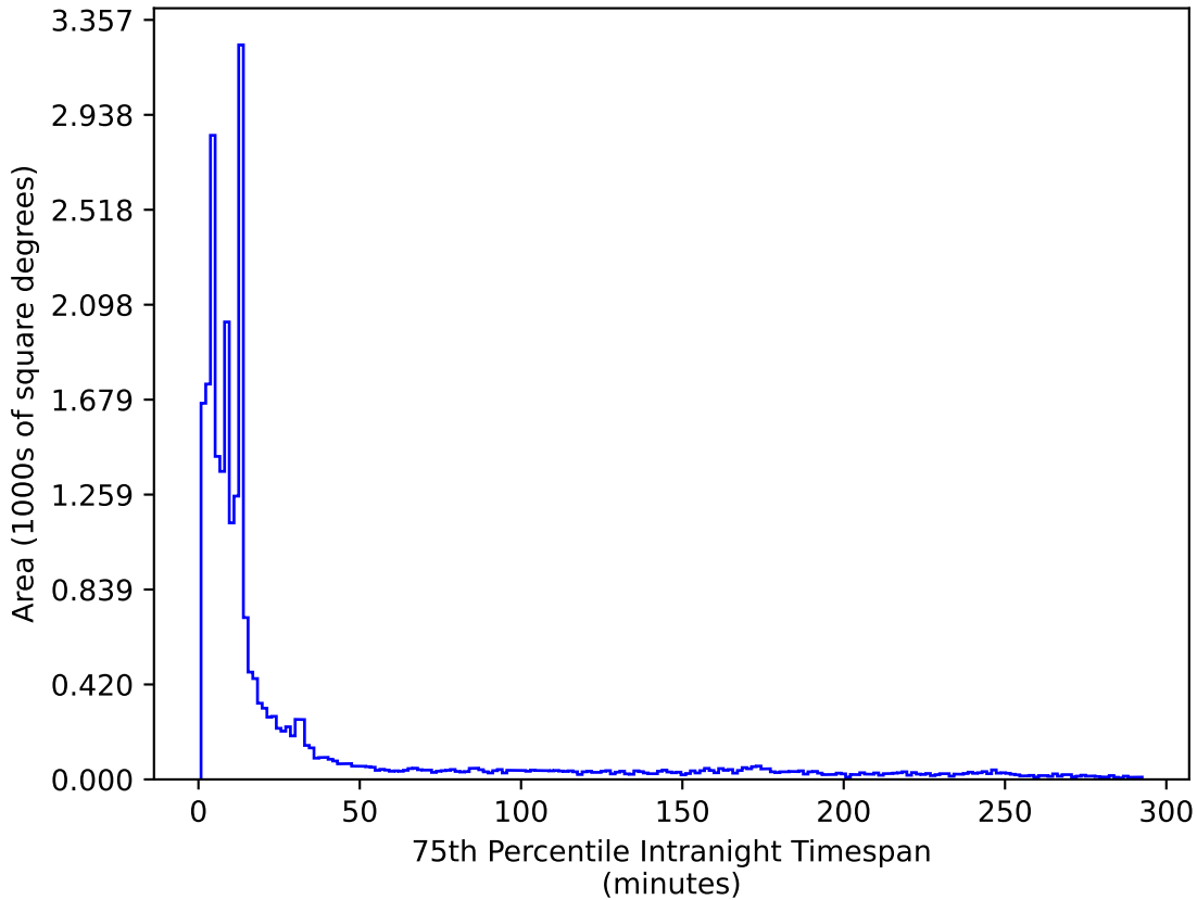
baseline_v3.0_10yrs All sky i band: 75th Percentile Intranight Timespan
