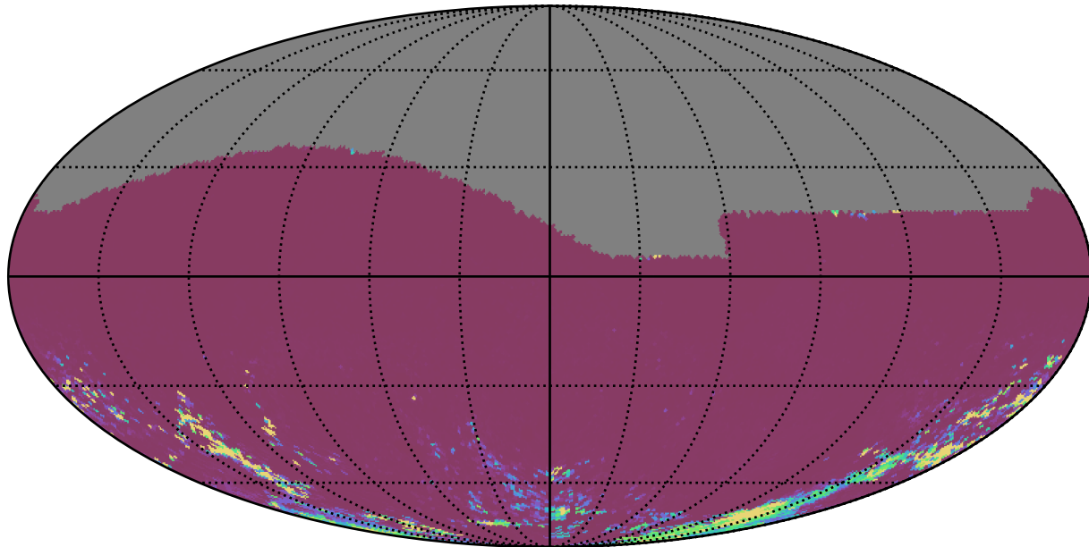
baseline_v3.0_10yrs All sky gr bands: 75th Percentile Intranight Timespan
