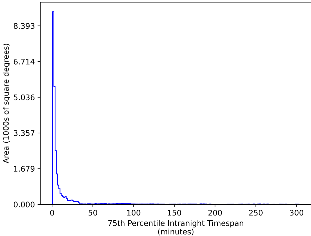
baseline_v3.0_10yrs All sky g band: 75th Percentile Intranight Timespan
