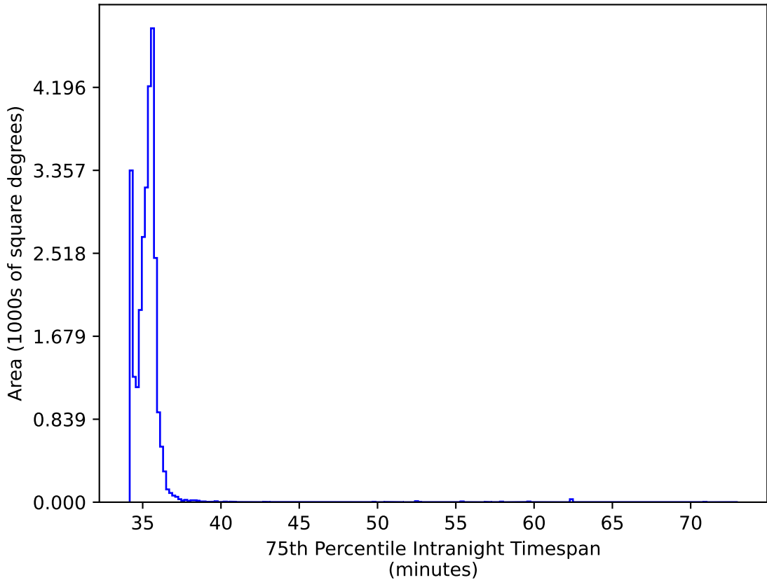
baseline_v3.0_10yrs All sky all bands: 75th Percentile Intranight Timespan
