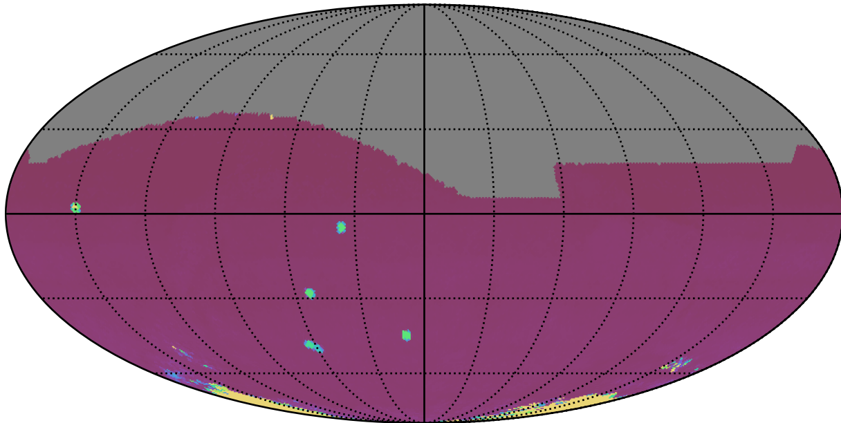
baseline_v3.0_10yrs All sky: 75th Percentile Intranight Timespan
