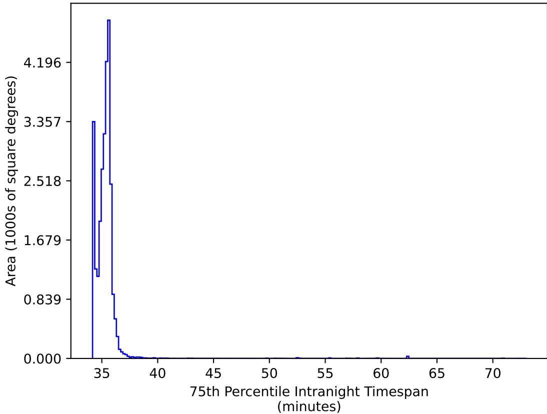
baseline_v3.0_10yrs All sky: 75th Percentile Intranight Timespan
