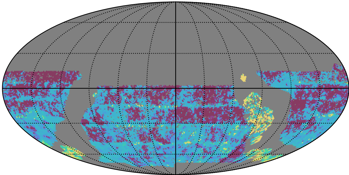
baseline_v3.0_10yrs WFD z band: 20thPercentile Inter-Night Gap
