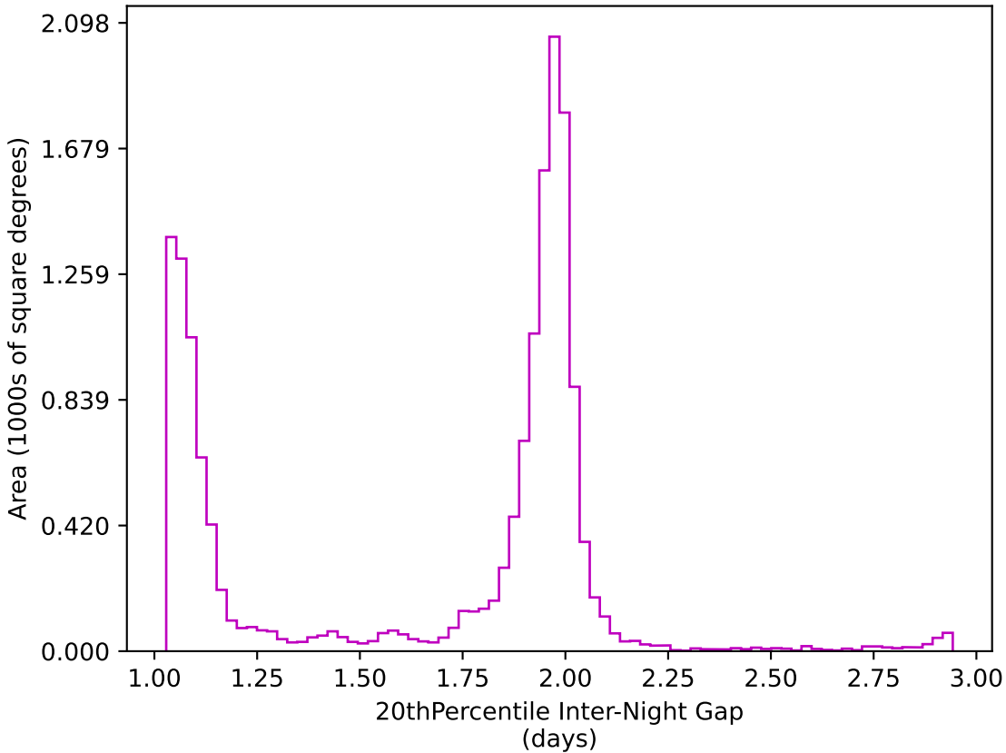
baseline_v3.0_10yrs WFD z band: 20thPercentile Inter-Night Gap
