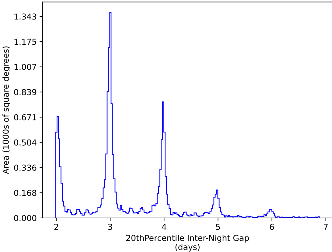
baseline_v3.0_10yrs WFD y band: 20thPercentile Inter-Night Gap
