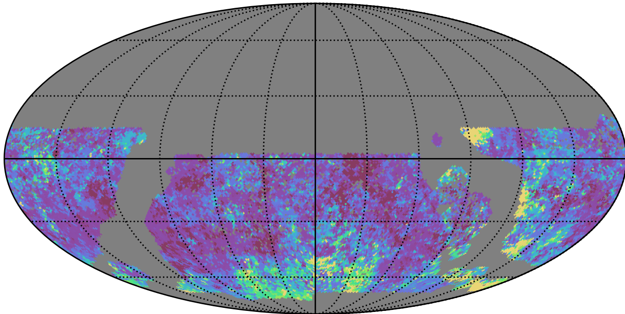
baseline_v3.0_10yrs WFD u band: 20thPercentile Inter-Night Gap
