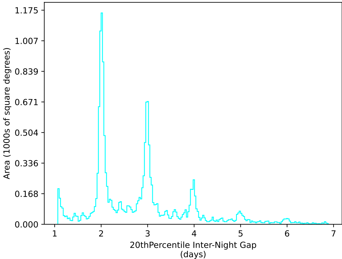
baseline_v3.0_10yrs WFD u band: 20thPercentile Inter-Night Gap
