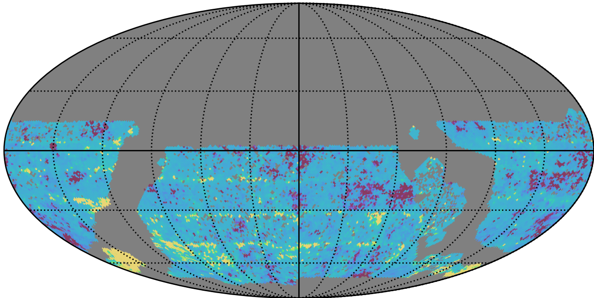
baseline_v3.0_10yrs WFD r band: 20thPercentile Inter-Night Gap
