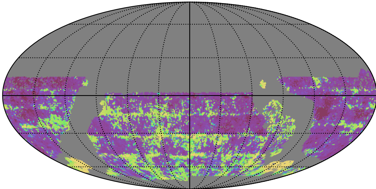
baseline_v3.0_10yrs WFD i band: 20thPercentile Inter-Night Gap
