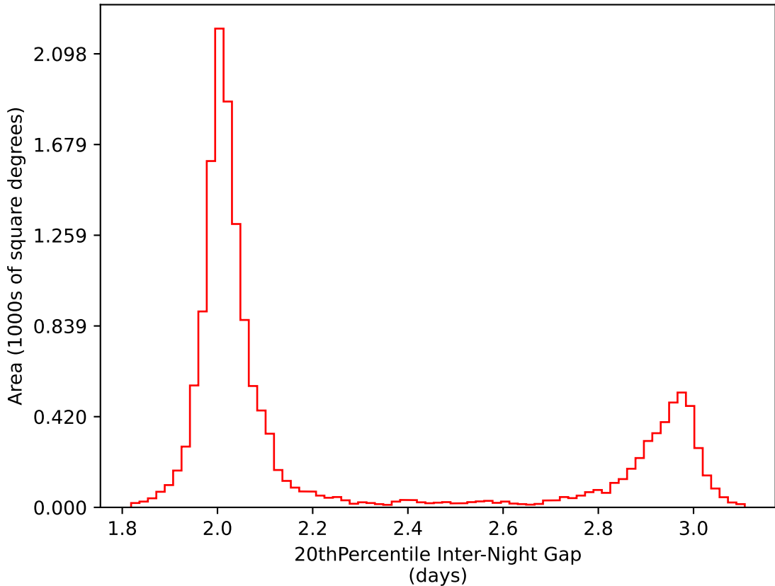
baseline_v3.0_10yrs WFD i band: 20thPercentile Inter-Night Gap
