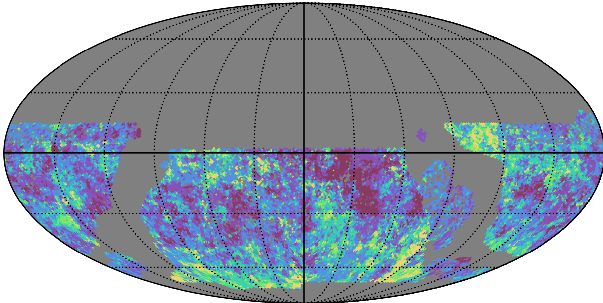
baseline_v3.0_10yrs WFD g band: 20thPercentile Inter-Night Gap
