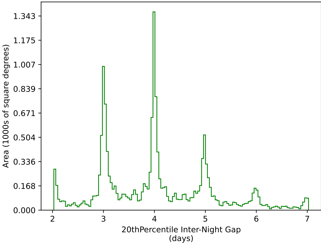
baseline_v3.0_10yrs WFD g band: 20thPercentile Inter-Night Gap
