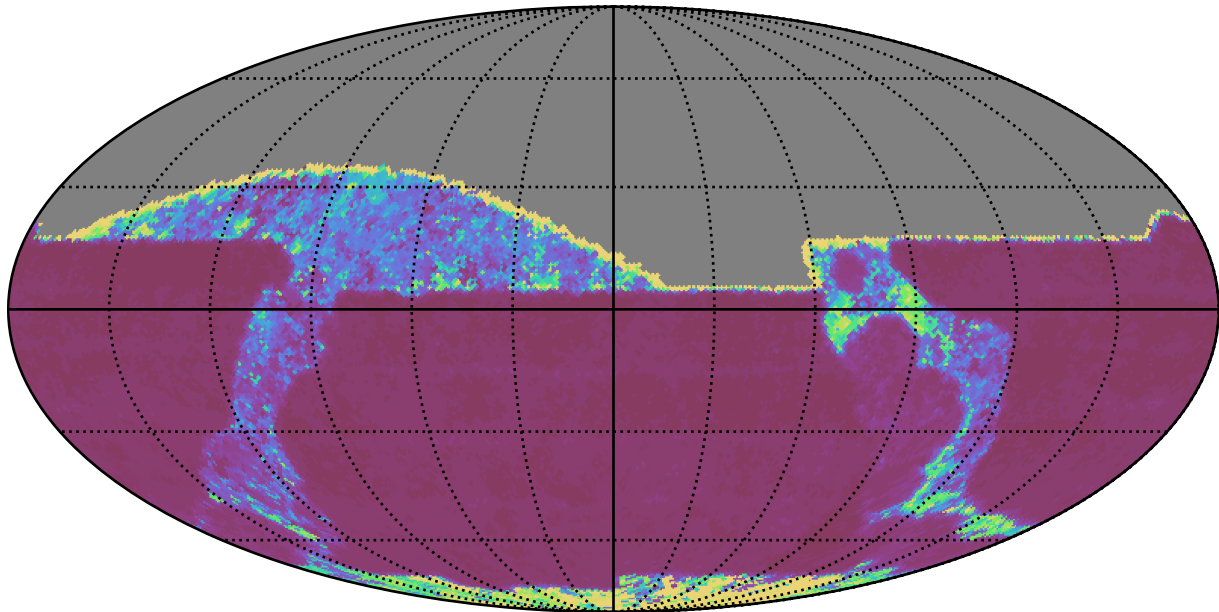
baseline_v3.0_10yrs All sky z band: 20thPercentile Inter-Night Gap
