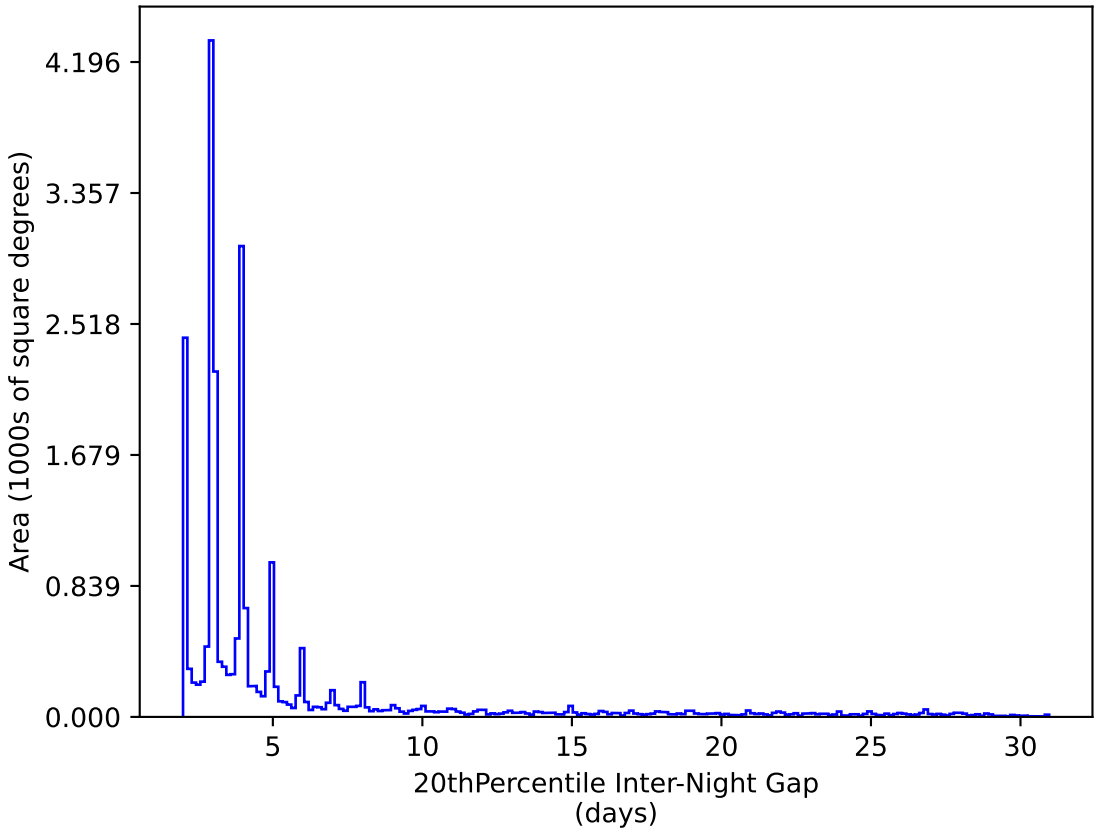
baseline_v3.0_10yrs All sky y band: 20thPercentile Inter-Night Gap
