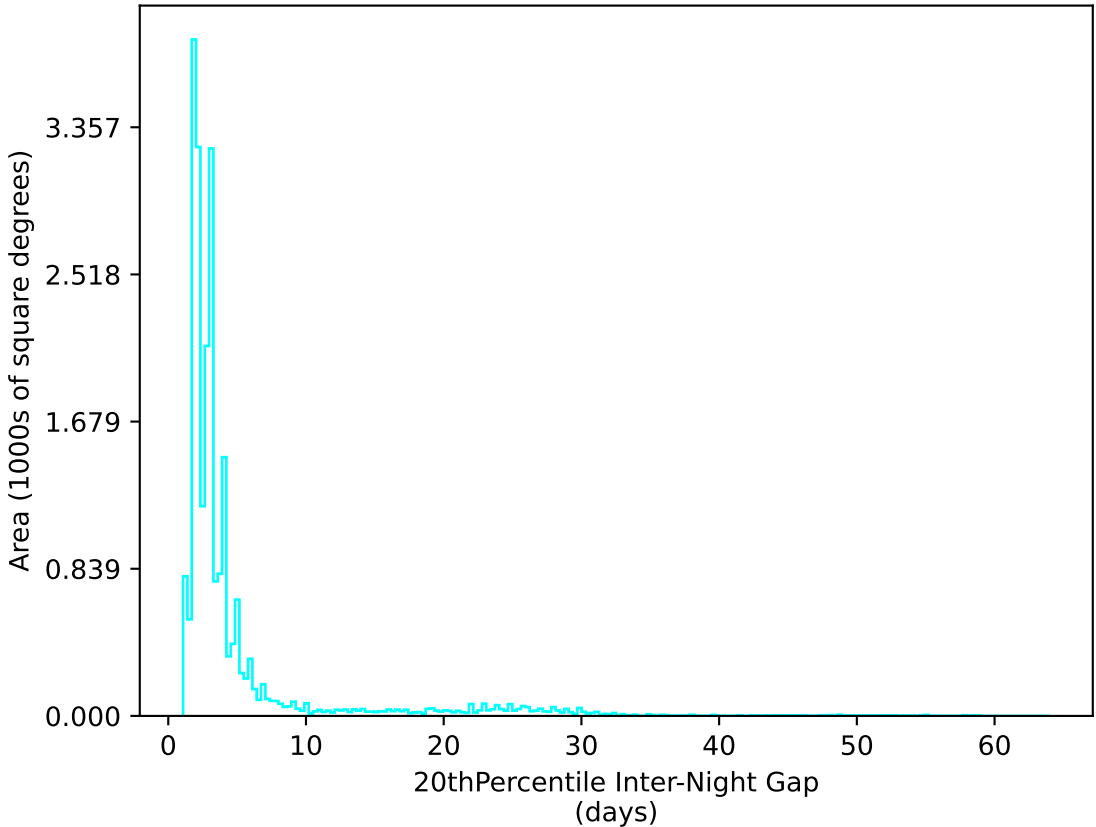
baseline_v3.0_10yrs All sky u band: 20thPercentile Inter-Night Gap
