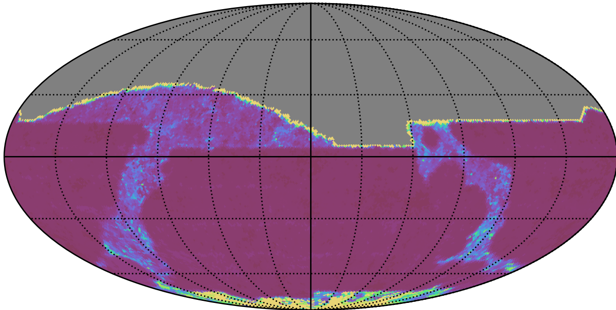
baseline_v3.0_10yrs All sky r band: 20thPercentile Inter-Night Gap
