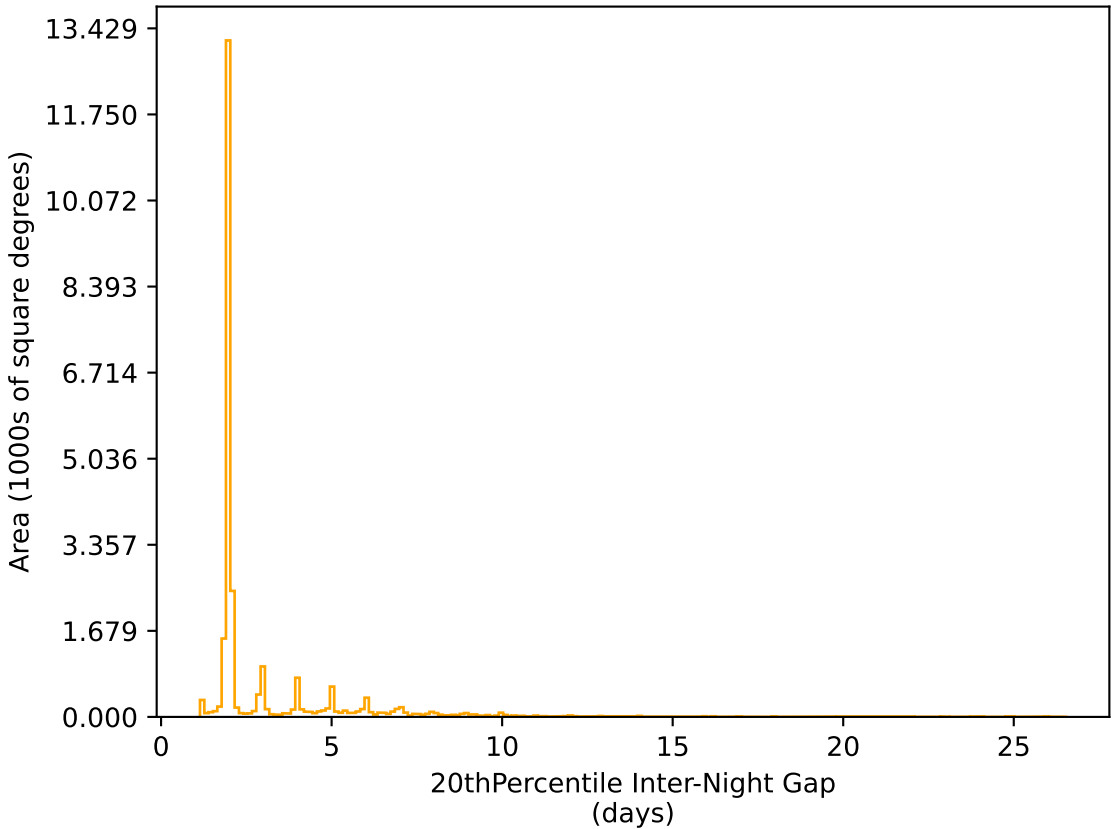
baseline_v3.0_10yrs All sky r band: 20thPercentile Inter-Night Gap
