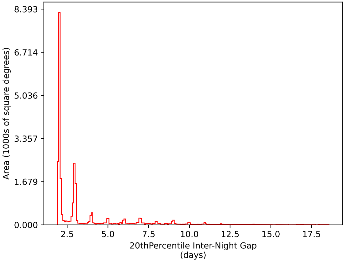
baseline_v3.0_10yrs All sky i band: 20thPercentile Inter-Night Gap
