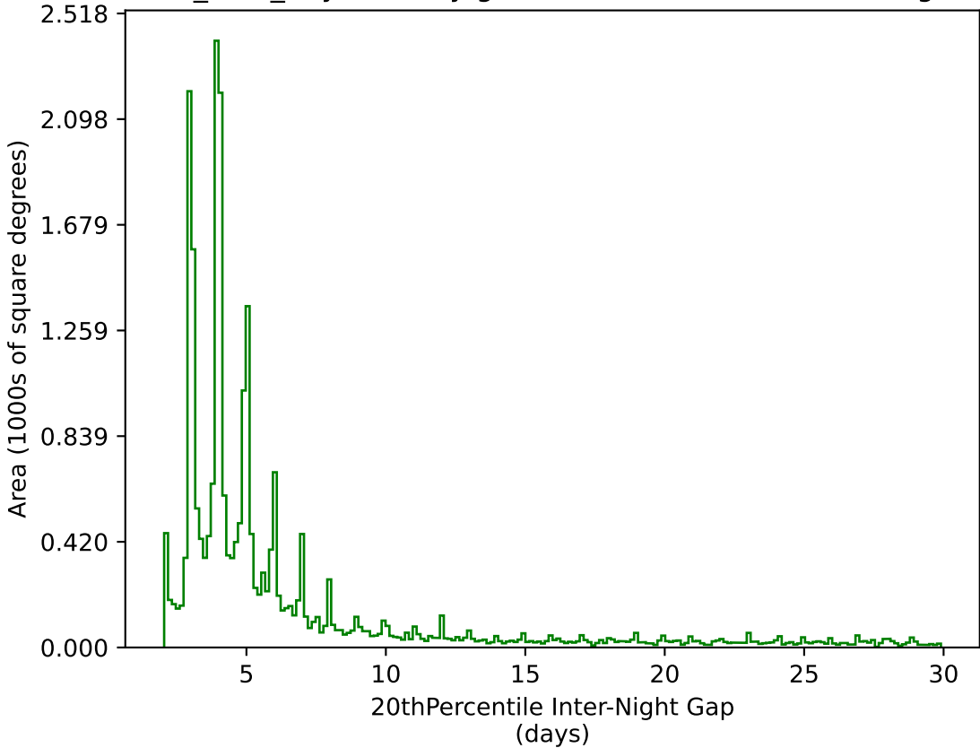
baseline_v3.0_10yrs All sky g band: 20thPercentile Inter-Night Gap
