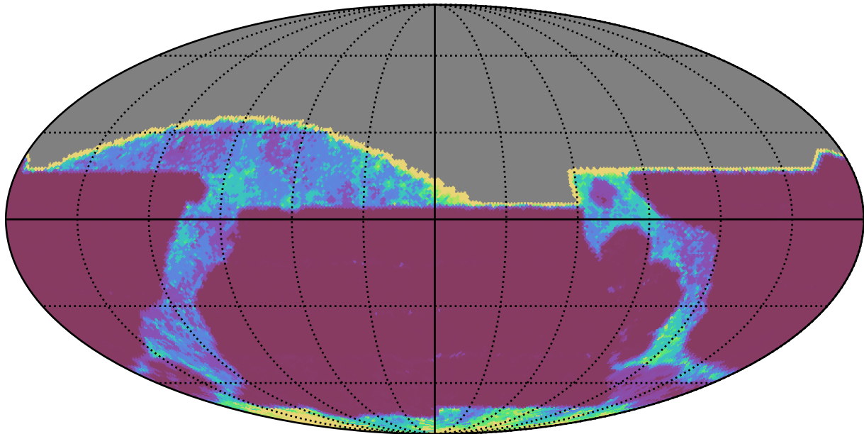
baseline_v3.0_10yrs All sky all bands: 20thPercentile Inter-Night Gap
