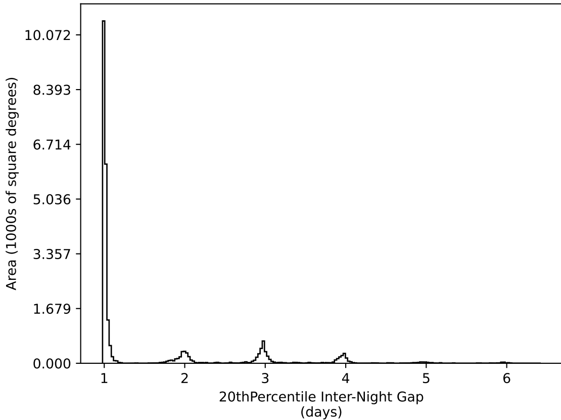
baseline_v3.0_10yrs All sky all bands: 20thPercentile Inter-Night Gap
