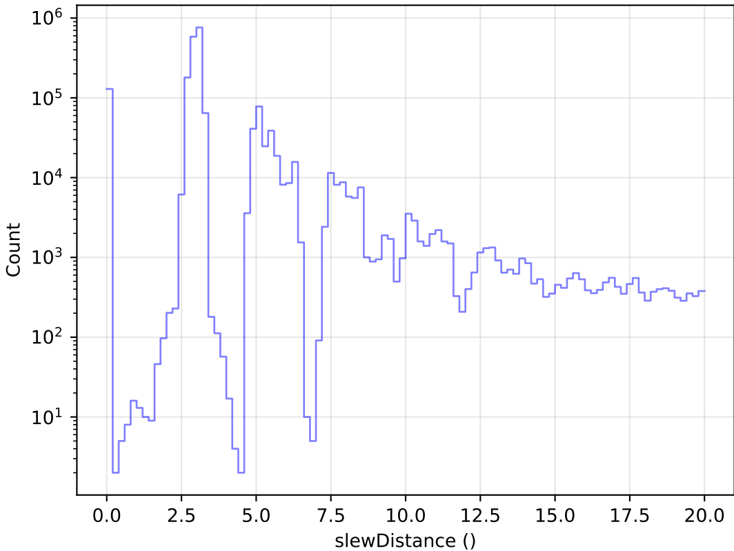
baseline_v3.0_10yrs All visits: Zoom Slew Distance Histogram
