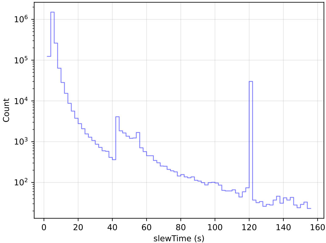
baseline_v3.0_10yrs All visits: Slew Time Histogram
