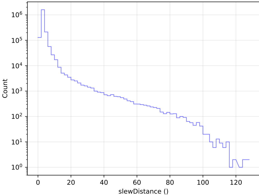
baseline_v3.0_10yrs All visits: Slew Distance Histogram
